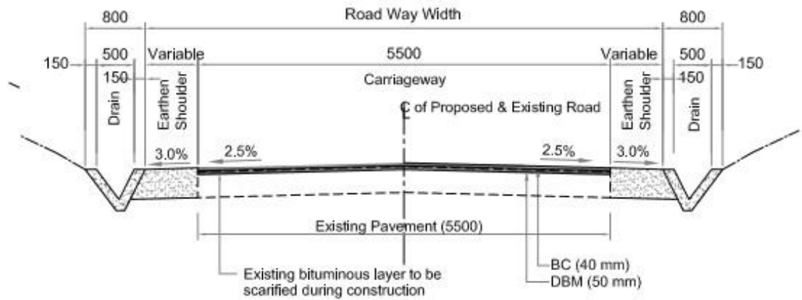
TCS-02 : Typical Cross section of Intermediate Lane Carriageway with Earthen Shoulder with Both Side RR Masonry Triangular Drain
