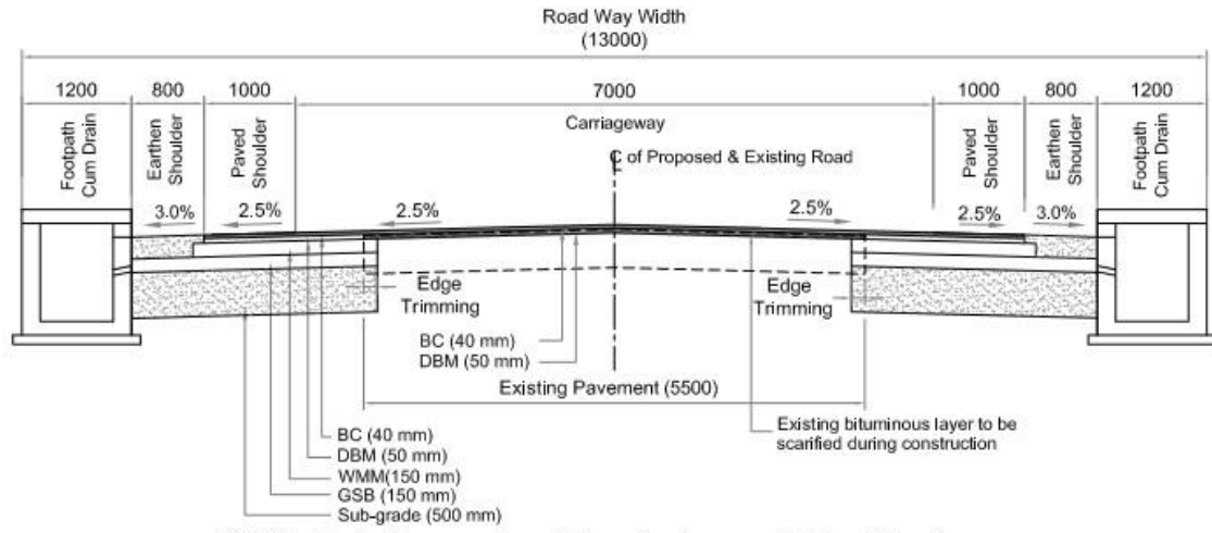
TCS-01 : Typical Cross section of 2-lane Carriageway with Paved Shoulder with Both Side Footpath cum RCC Rectangular Drain
